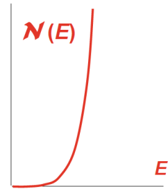
Unbound spectrum
