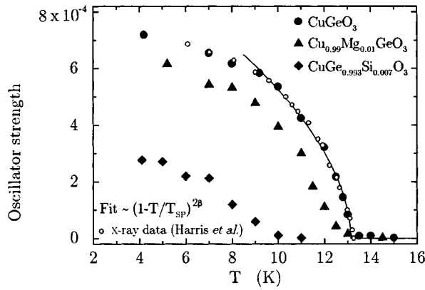
FIG. 3. Temperature dependence of the oscillator strength of the zone-boundary mode observed for E\parallel b at 800\text{ cm}^{-1} on pure (filled circles), 1% Mg-doped (triangles), and 0.7% Si-doped (diamonds) \text{CuGeO}_3 single crystals. For comparison the x-ray scattering data of Harris et al. (Ref. 14) are also plotted (open circles).
