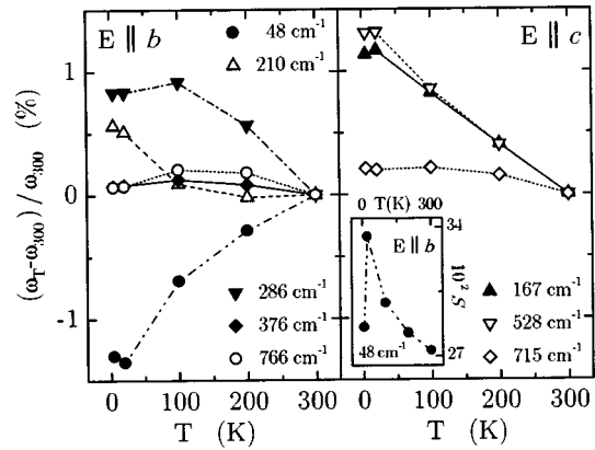
FIG. 4. Temperature dependence of the frequency shift (in percent) of the transverse optical phonons observed for E\parallel b and E\parallel c on the pure single crystal of \text{CuGeO}_3 . In the inset the oscillator strength S of the mode detected at 48\text{ cm}^{-1} , for E\parallel b , is plotted versus the temperature.
