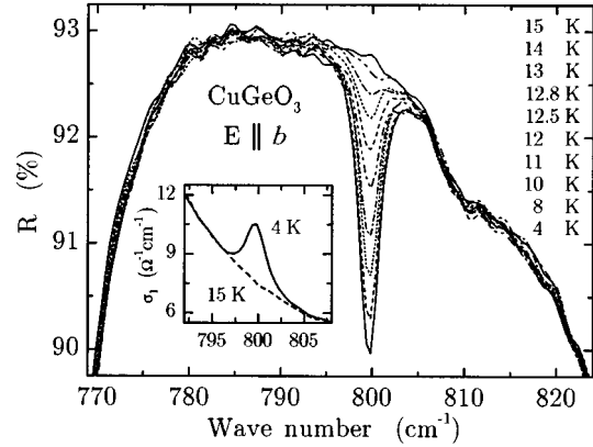
FIG. 2. Detailed temperature dependence of the feature observed with E||b in the reflectivity spectra at 800\text{ cm}^{-1} for T < T_{\text{SP}} . In the inset, where the dynamical conductivity calculated via Kramers-Kronig analysis is plotted, a new peak is clearly visible for T=4\text{ K} .
