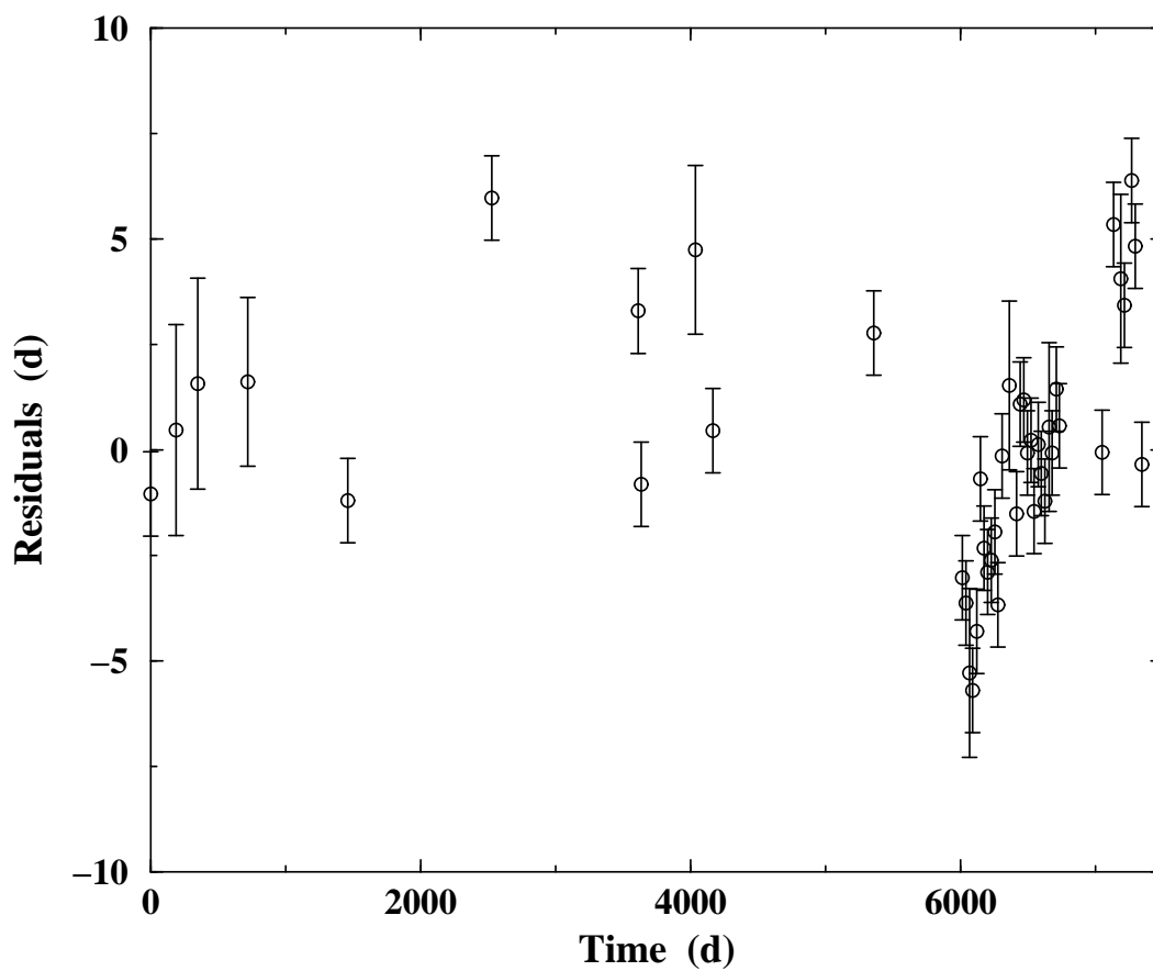
Fig. 2.— The timing residuals assuming a single period for all of the data, hypothesis H_1 .
