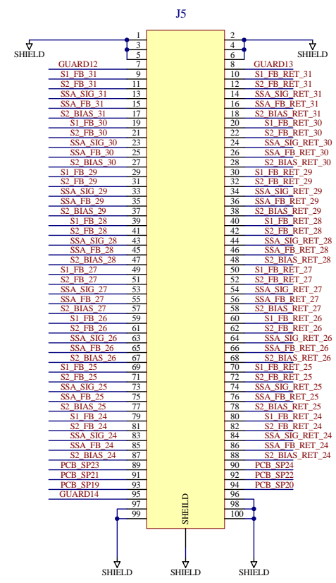
Gold Dot Connector Pads Locate on Bottom of Board
